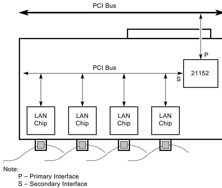
Figure 1-2. 21152 with Option Cards
