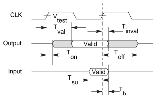
Figure 15-2. PCI Signal Timing Measurement Conditions
