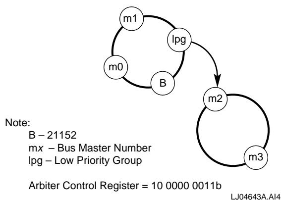
Figure 9-1. Secondary Arbiter Example
