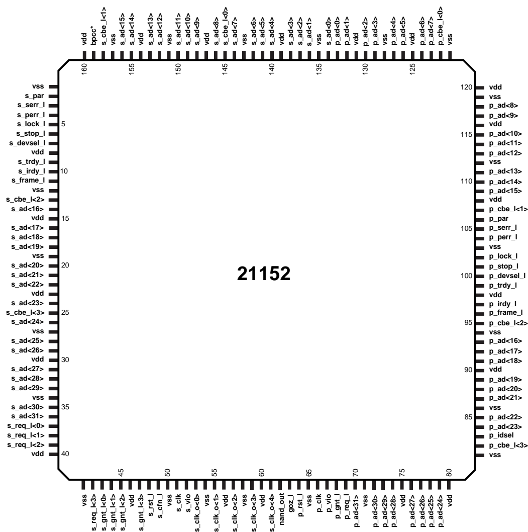
Figure 3-1. 21152 Pinout Diagram
