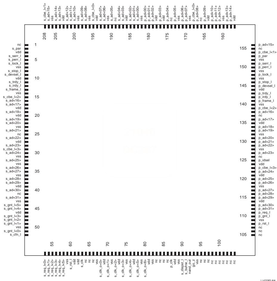
Figure 2-1. 21050 Pinout Diagram
