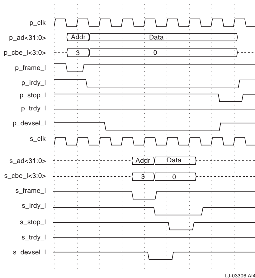
Figure 4-11. I/O Write with Target Abort
