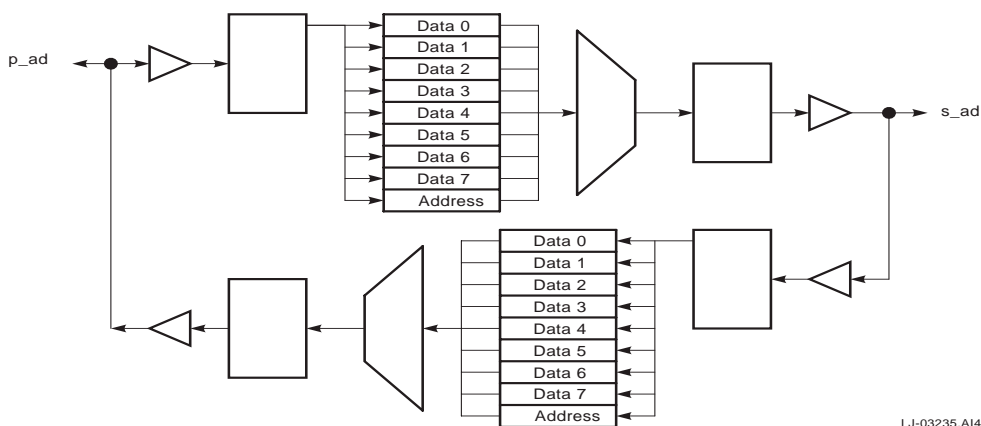
Figure 4-1. 21050 Data Path
