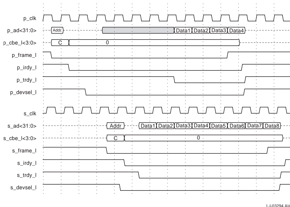
Figure 4-6. Memory Read multiple with Extra Prefetching
