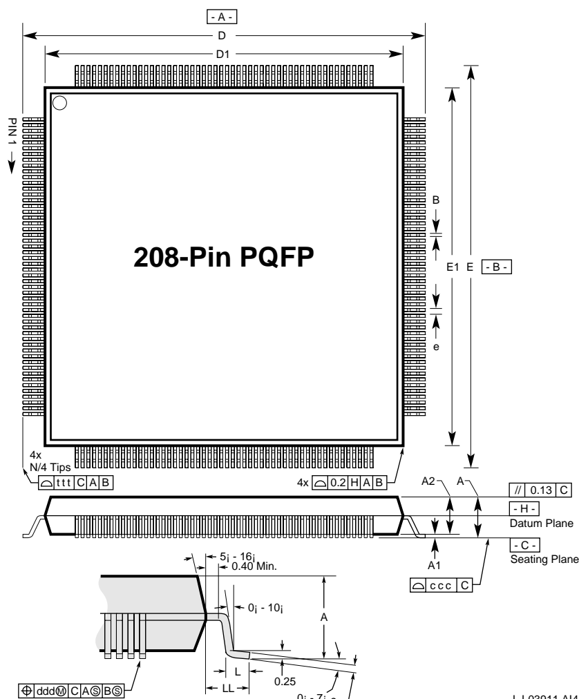
Figure 7-1. Package Dimensions
