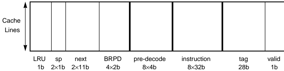
FIGURE A-4 Simplified I-cache Organization (Only 1 Set Shown)
