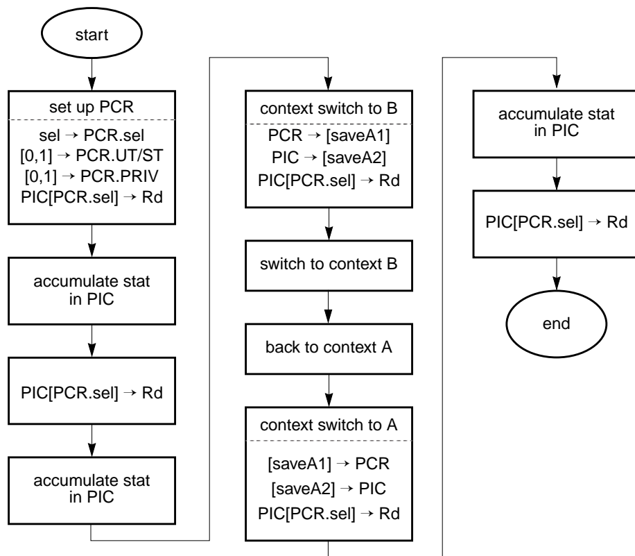
FIGURE B-3 PCR/PIC Operational Flow
