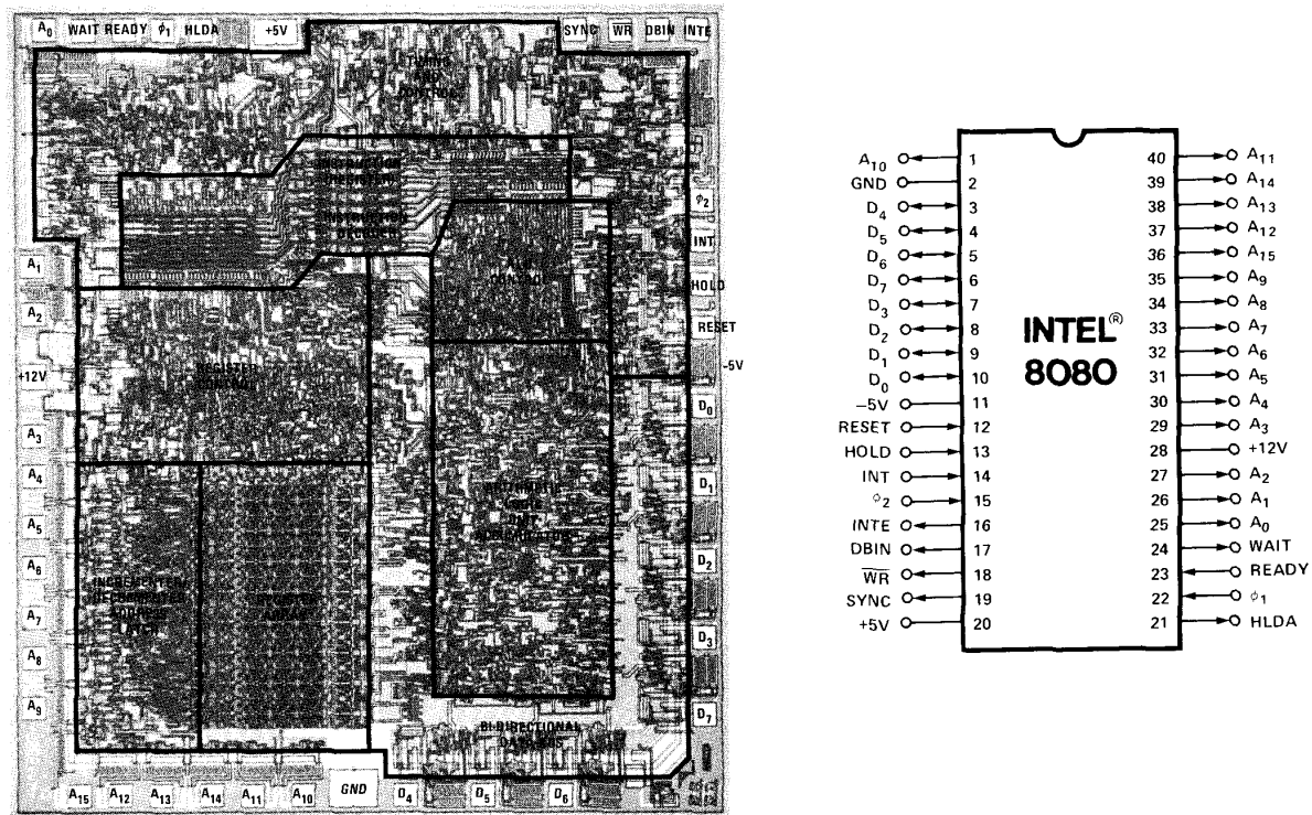
Figure 2-1. 8080 Photomicrograph With Pin Designations
