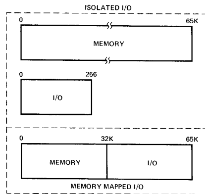
Figure 3-8. Memory/I/O Mapping.
