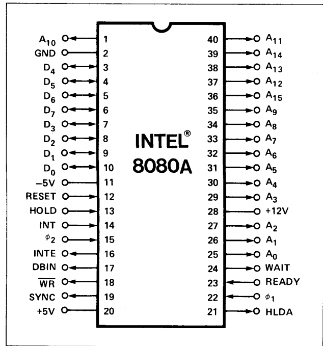
Pin Configuration
