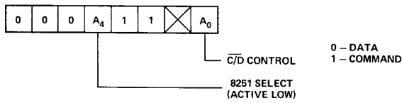
Figure 3-13. 8251 Format.
