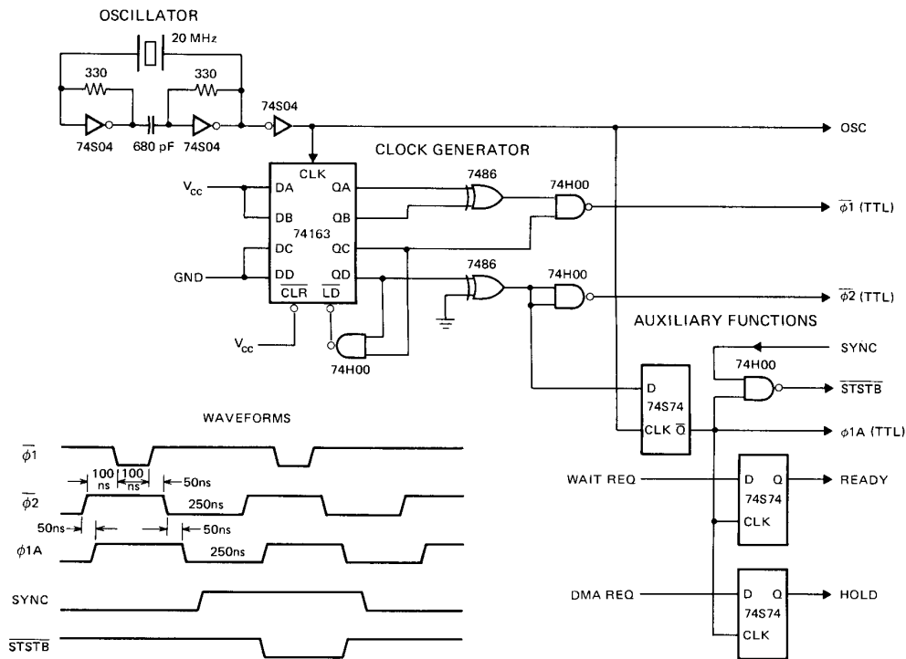
Figure 3-3. 8080 Clock Generator
