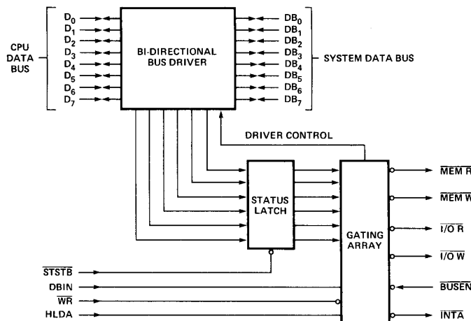
8228 BLOCK DIAGRAM
