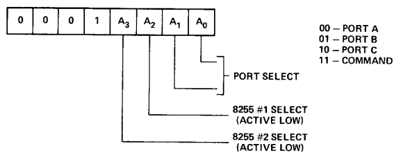
Figure 3-14. 8255 Format.
