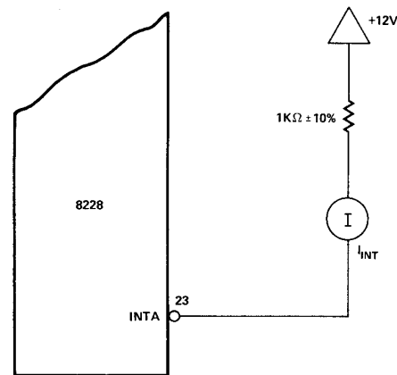
INTA Test Circuit (for RST 7)
