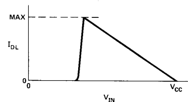
DATA BUS CHARACTERISTIC DURING DBIN
