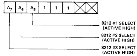
Figure 3-15. 8212 Format.
