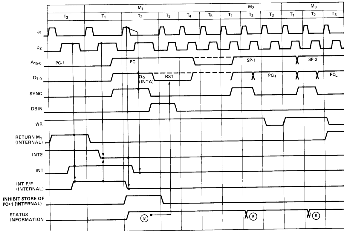
Figure 2-8. Interrupt Timing
