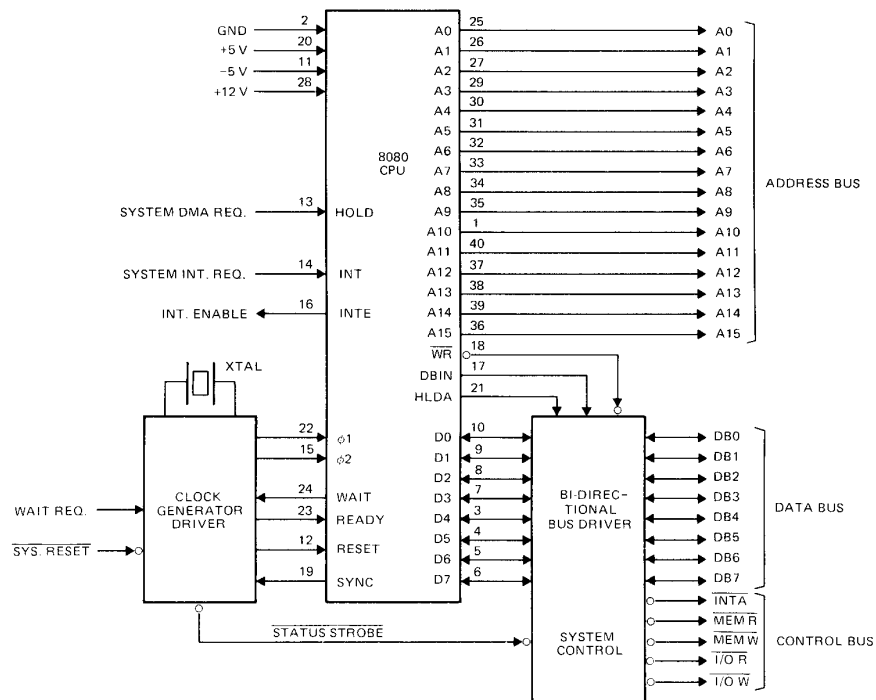
Figure 3-2. 8080 CPU Interface
