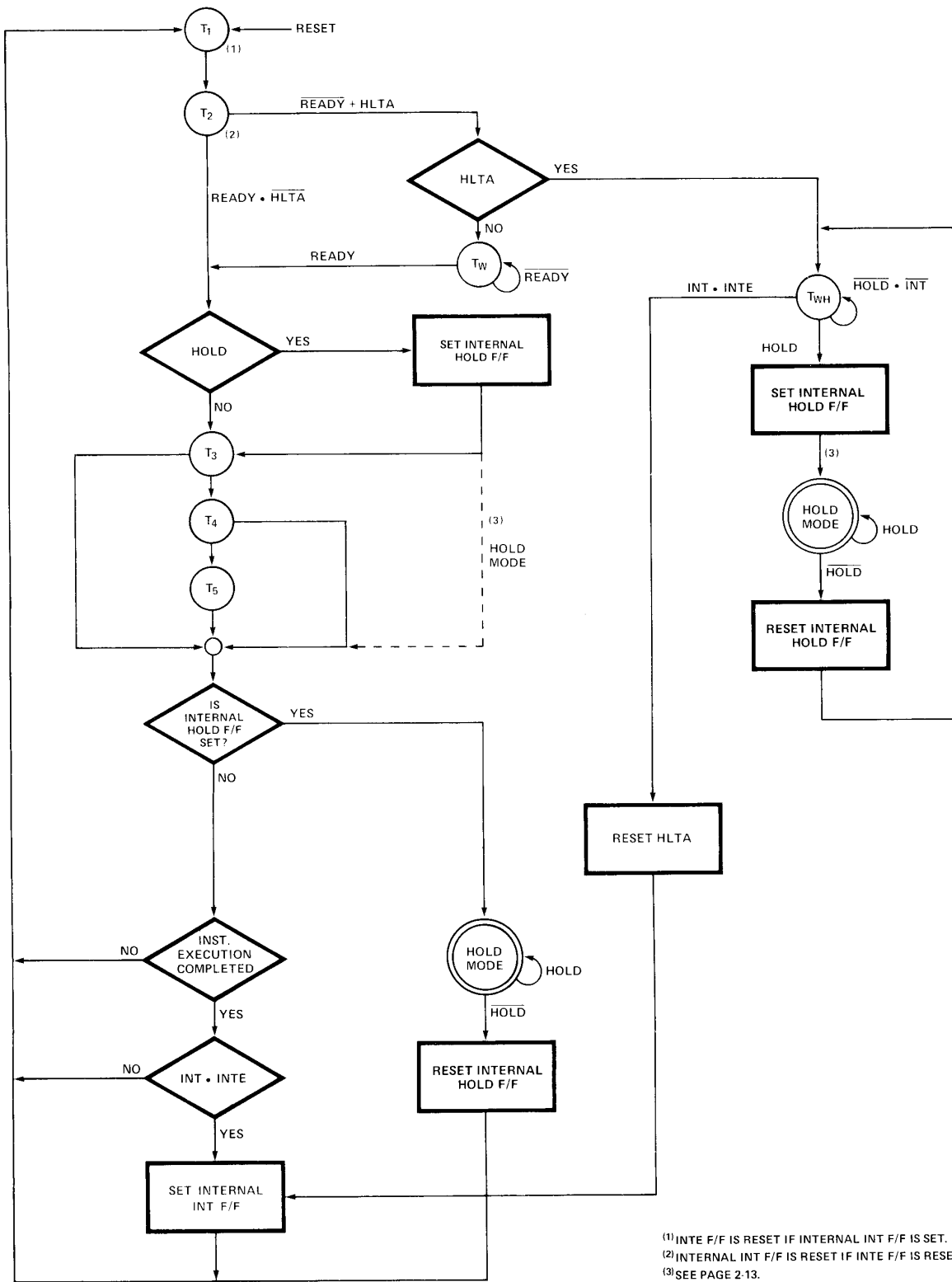
Figure 2-4. CPU State Transition Diagram
