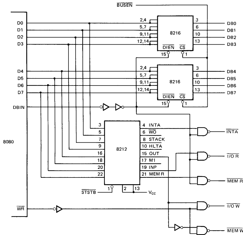
Figure 3-5. 8080 System Control
