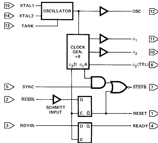
BLOCK DIAGRAM
