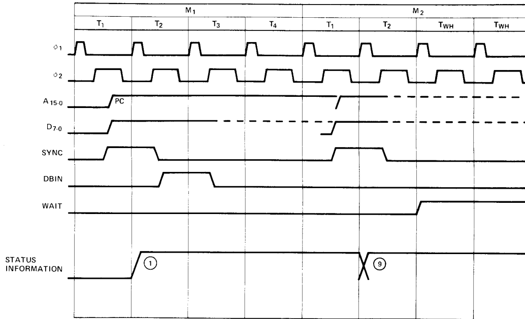
Figure 2-11. HALT Timing
