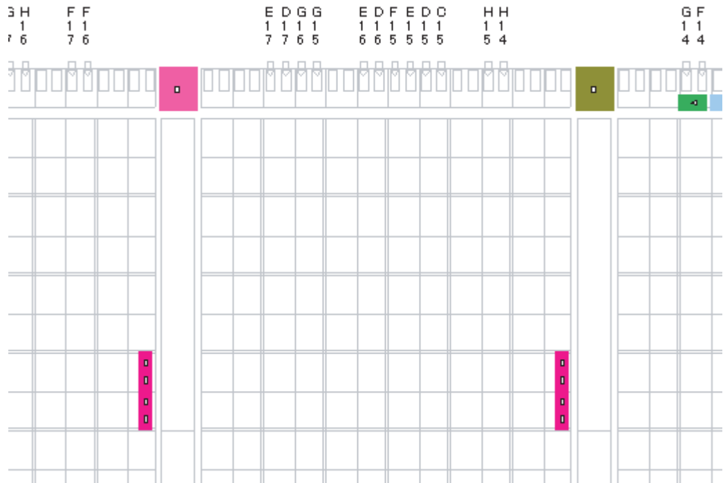
Figure 2-18: Top MGT Comma Control Flip-Flop Ideal Locations
