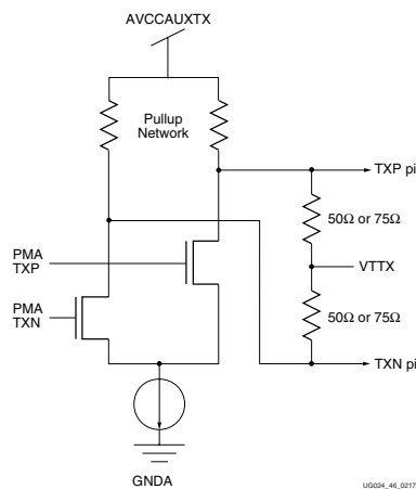
Figure 3-1: Differential Amplifier
