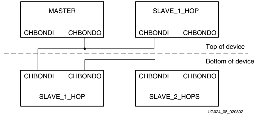
Figure 4-1: XC2VP2 Implementation
