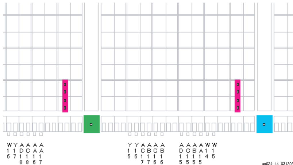
Figure 2-19: Bottom MGT Comma Control Flip-Flop Ideal Locations
