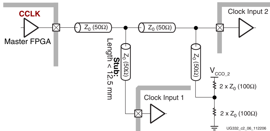
Figure 2-4: Multi-Drop: Master CCLK Output Drives Two Clock Inputs
