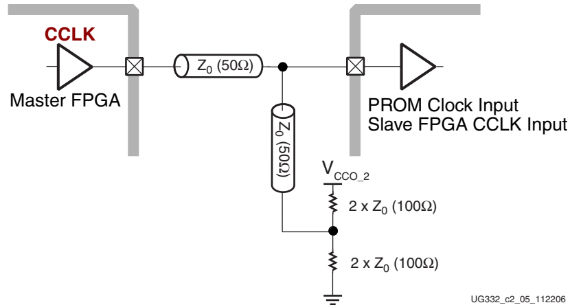
Figure 2-3: Point-to-Point: Master CCLK Output Drives Single Clock Load
