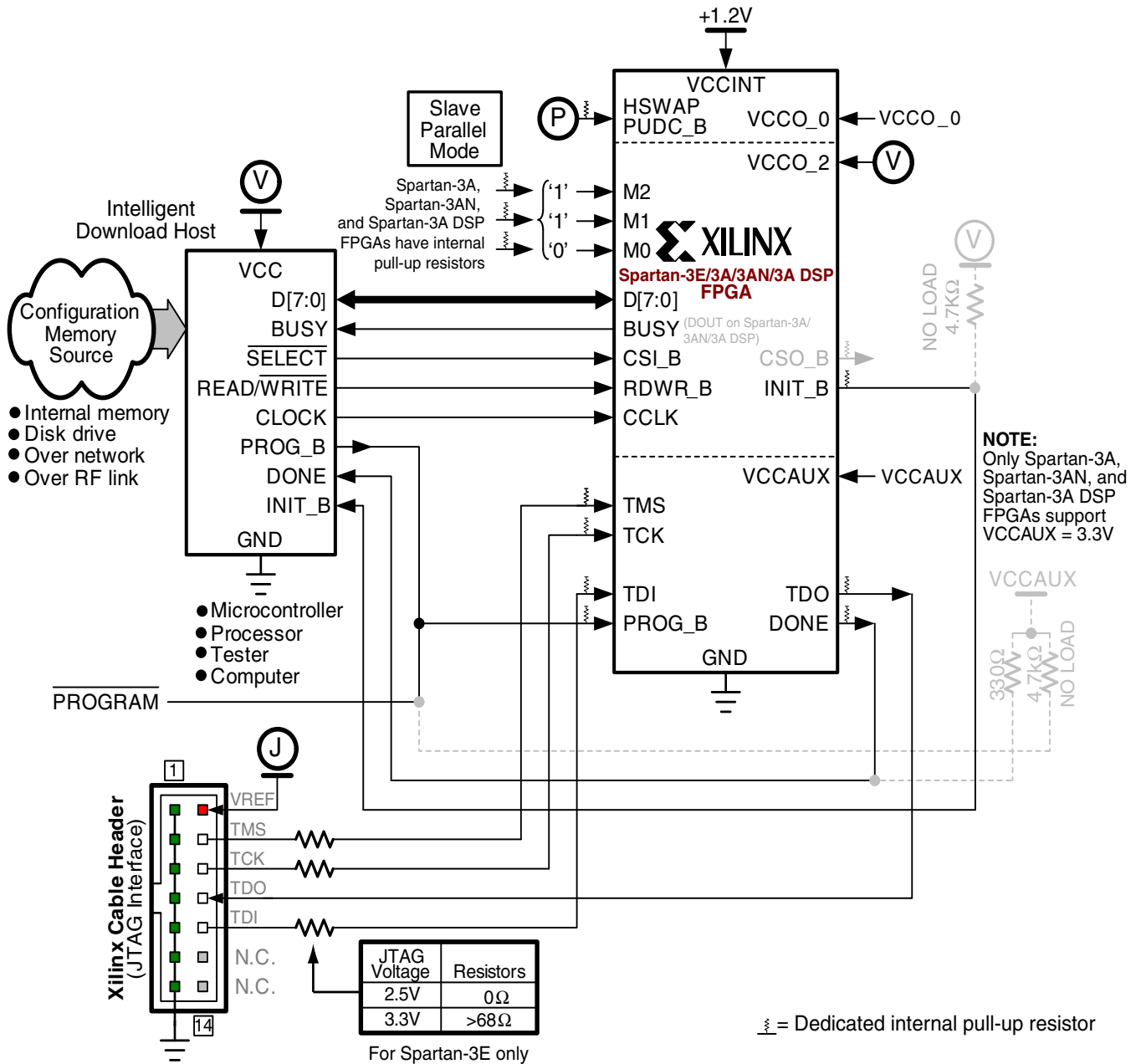
Figure 7-1: Slave Parallel Mode (Spartan-3E and Extended Spartan-3A FPGA Families)
