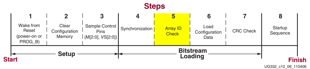
Figure 12-8: Check Array ID
