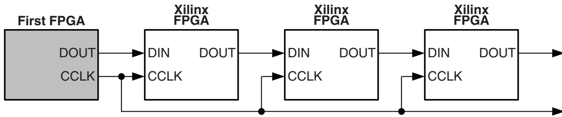
(a) Serial Daisy Chain (using Slave Serial mode)
