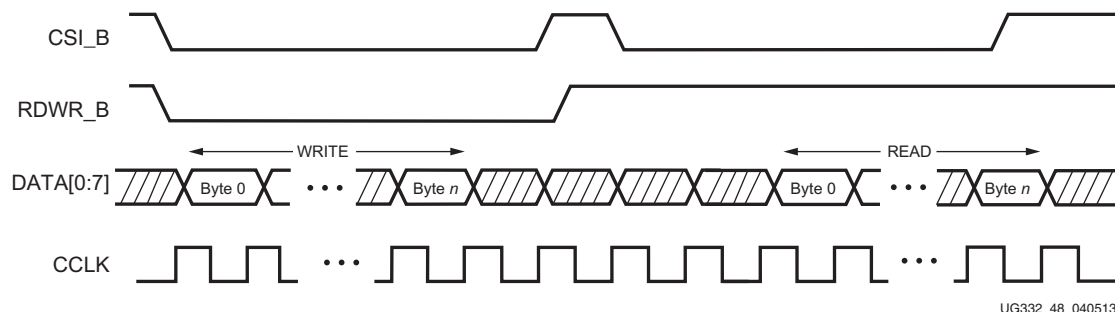
Figure 18-1: Changing the SelectMAP Port from Write to Read Control
