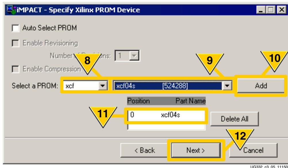
Figure 3-10: Select Platform Flash PROM
