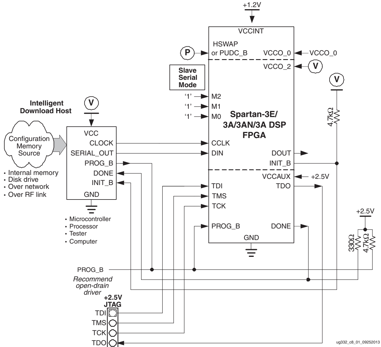
Figure 8-1: Slave Serial Configuration
