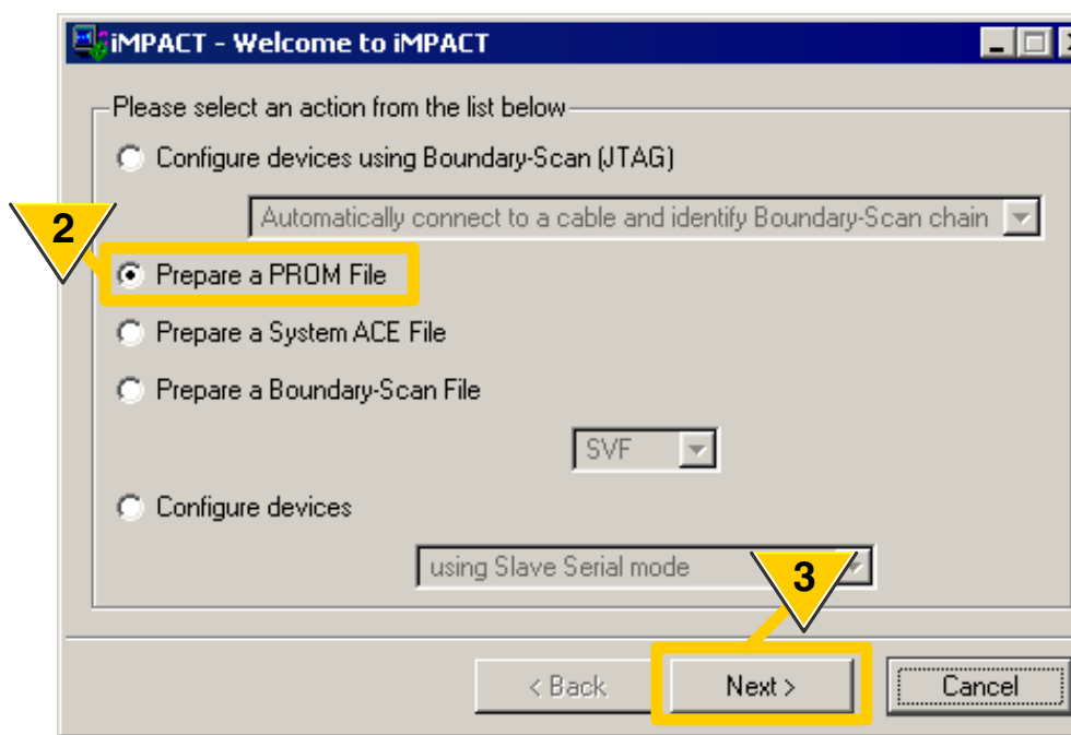
Figure 3-8: Prepare a PROM File
