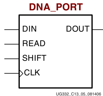
Figure 13-5: DNA_PORT Primitive (only available on Extended Spartan-3A Family FPGAs)
