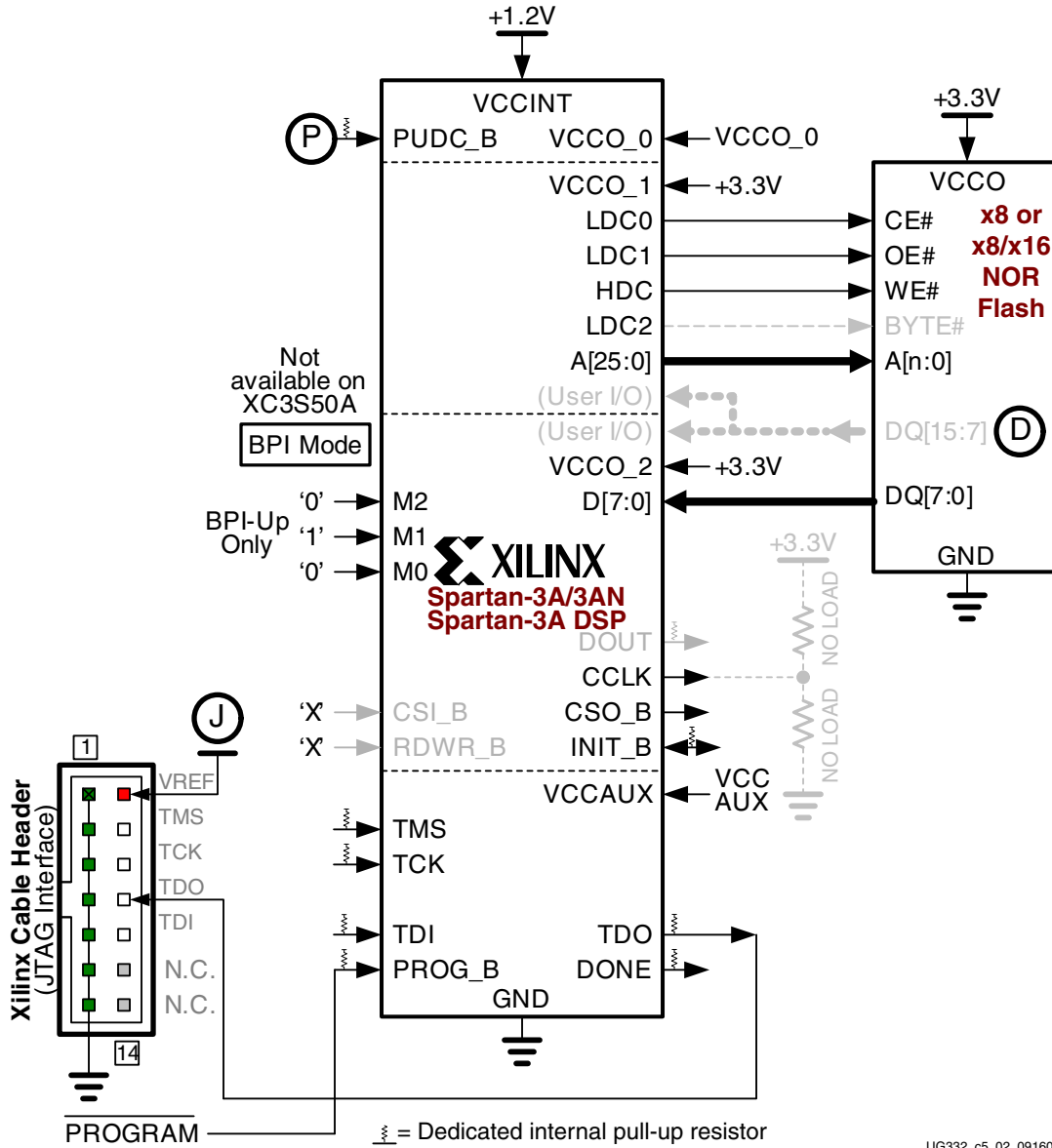
Figure 5-2: Extended Spartan-3A Family FPGA Configured from Parallel NOR Flash
