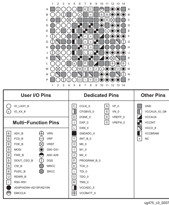
Figure 3-5: FTGB196 Package—XC7S6, XC7S15, XA7S6, and XA7S15 Pinout Diagram
