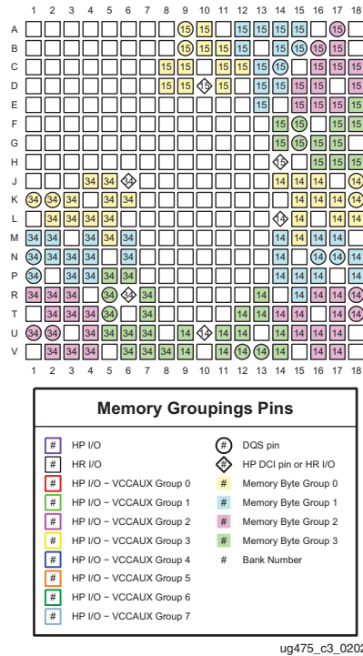
Figure 3-55: CSG325 Package—XC7A12T and XA7A12T Memory Groupings
