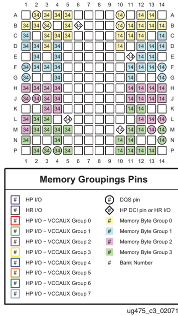
Figure 3-7: FTGB196 Package—XC7S6, XC7S15, XA7S6, and XA7S15 Memory Groupings
