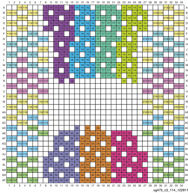
Figure 3-158: FF1158, FFG1158, FV1158, and RF1158 Packages—XC7VX415T, XC7VX550T, and XC7VX690T I/O Banks
