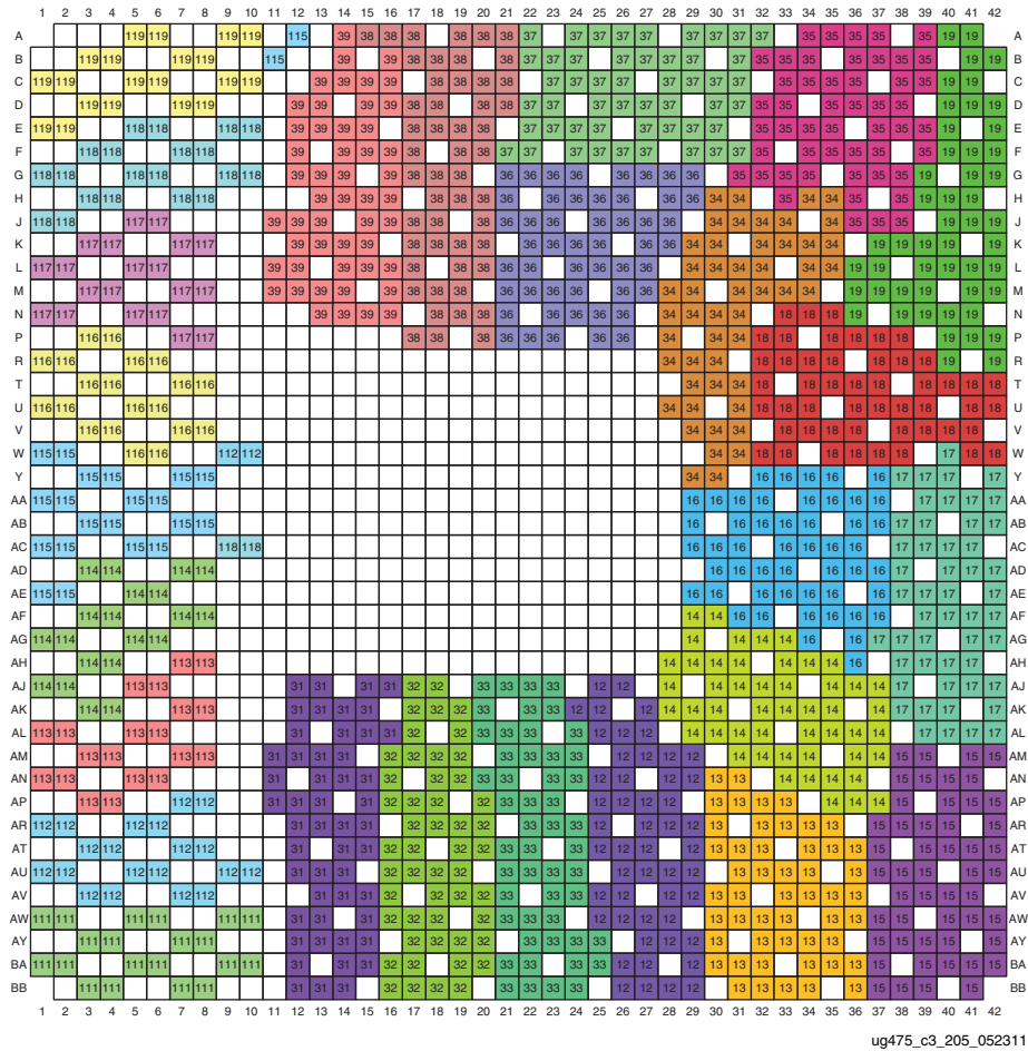
Figure 3-146: FH1761 and FHG1761 Packages—XC7V200T I/O Banks
