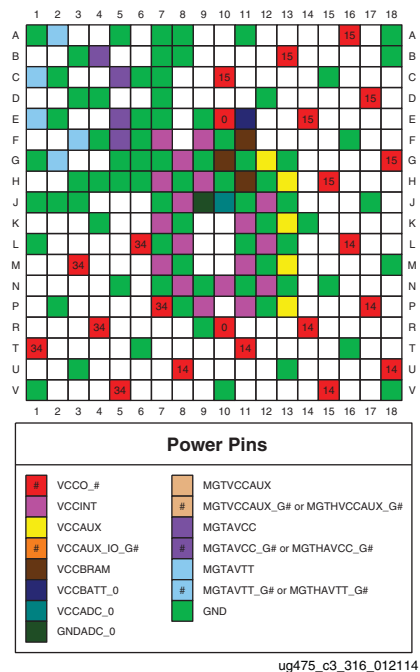
Figure 3-64: CS325 and CSG325 Packages—XC7A15T, XC7A35T, and XC7A50T CSG325 Packages (only)—XA7A15T, XA7A35T, and XA7A50T Power and GND Placement
