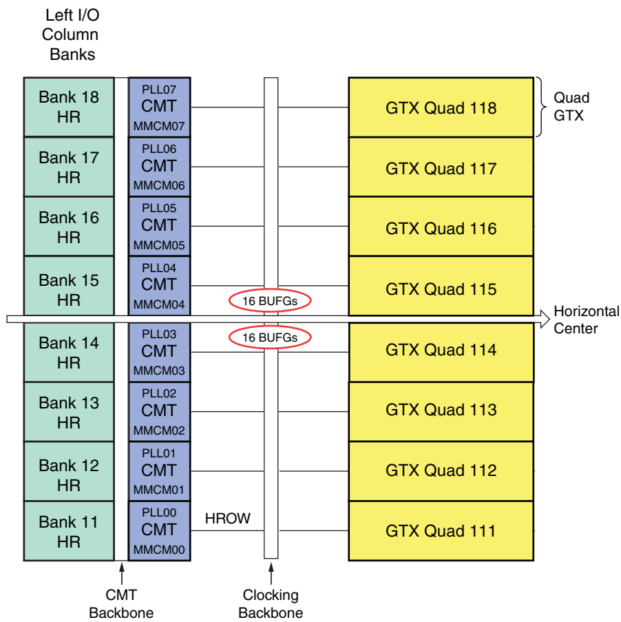
Figure 1-16: XC7K420T Banks
