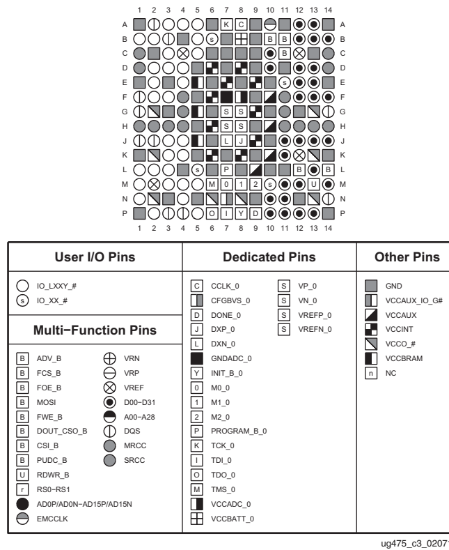
Figure 3-9: FTGB196 Package—XC7S25, XC7S50, XA7S25, and XA7S50 Pinout Diagram
