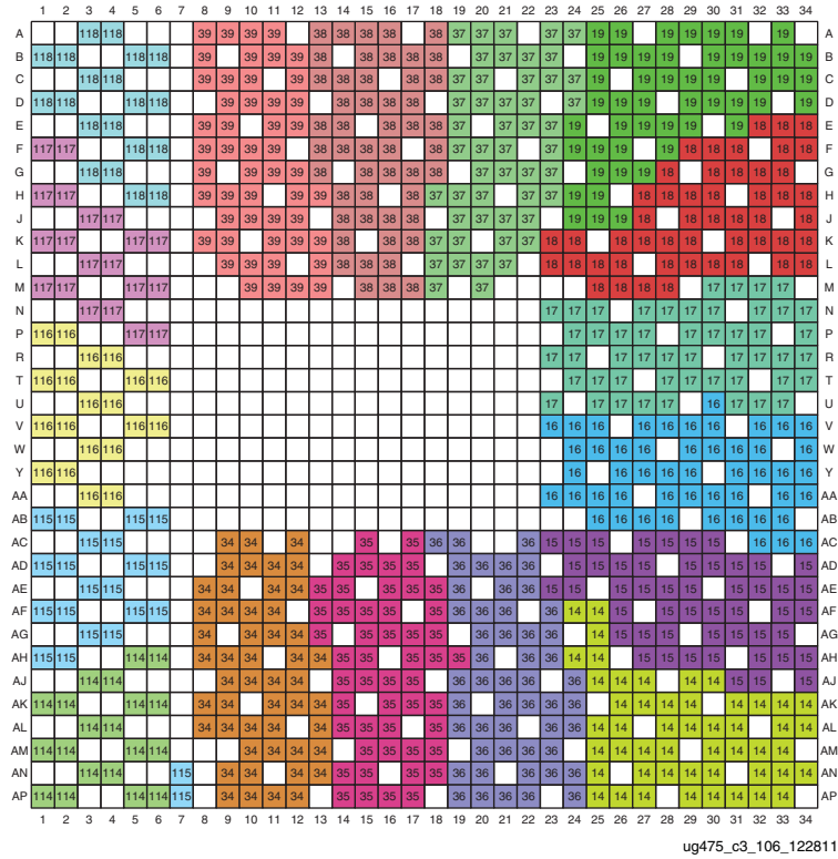
Figure 3-150: FF1157, FFG1157, and RF1157 Packages—XC7VX330T, XC7VX415T, and XC7VX690T I/O Banks
