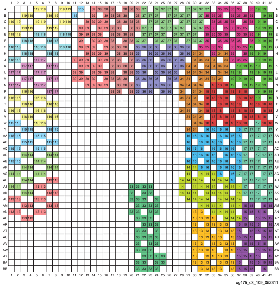
Figure 3-174: FF1761, FFG1761, and RF1761 Packages—XC7VX485T I/O Banks
