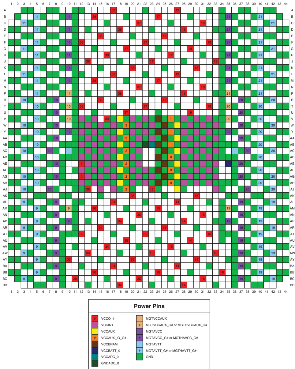
Figure 3-196: FF1927 and FFG1927 Packages—XC7VX550T and XC7VX690T Power and GND Placement
