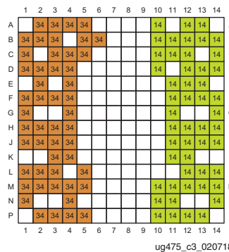
Figure 3-6: FTGB196 Package—XC7S6, XC7S15, XA7S6, and XA7S15 I/O Banks
