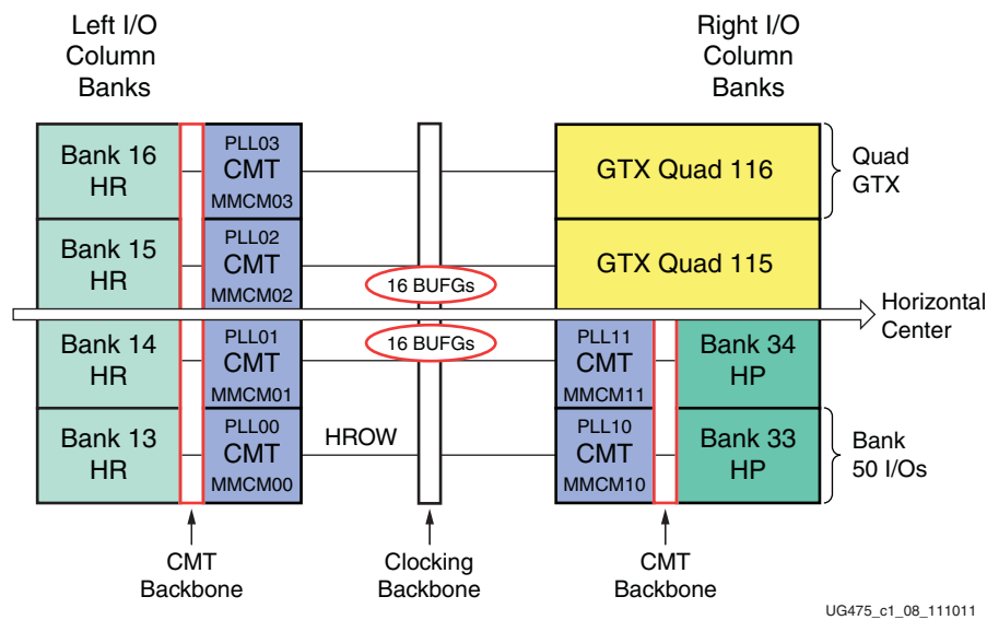
Figure 1-11: XC7K70T Banks
