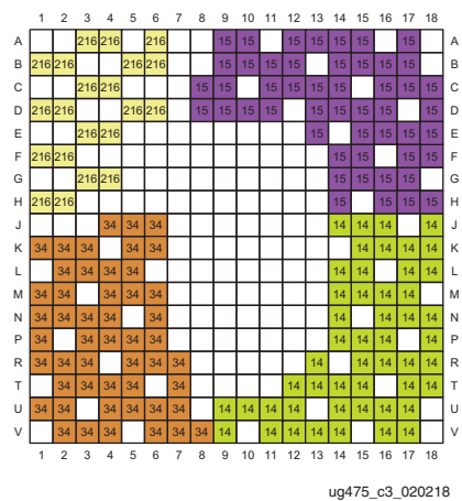
Figure 3-58: CSG325 Package—XC7A25T and XA7A25T I/O Banks
