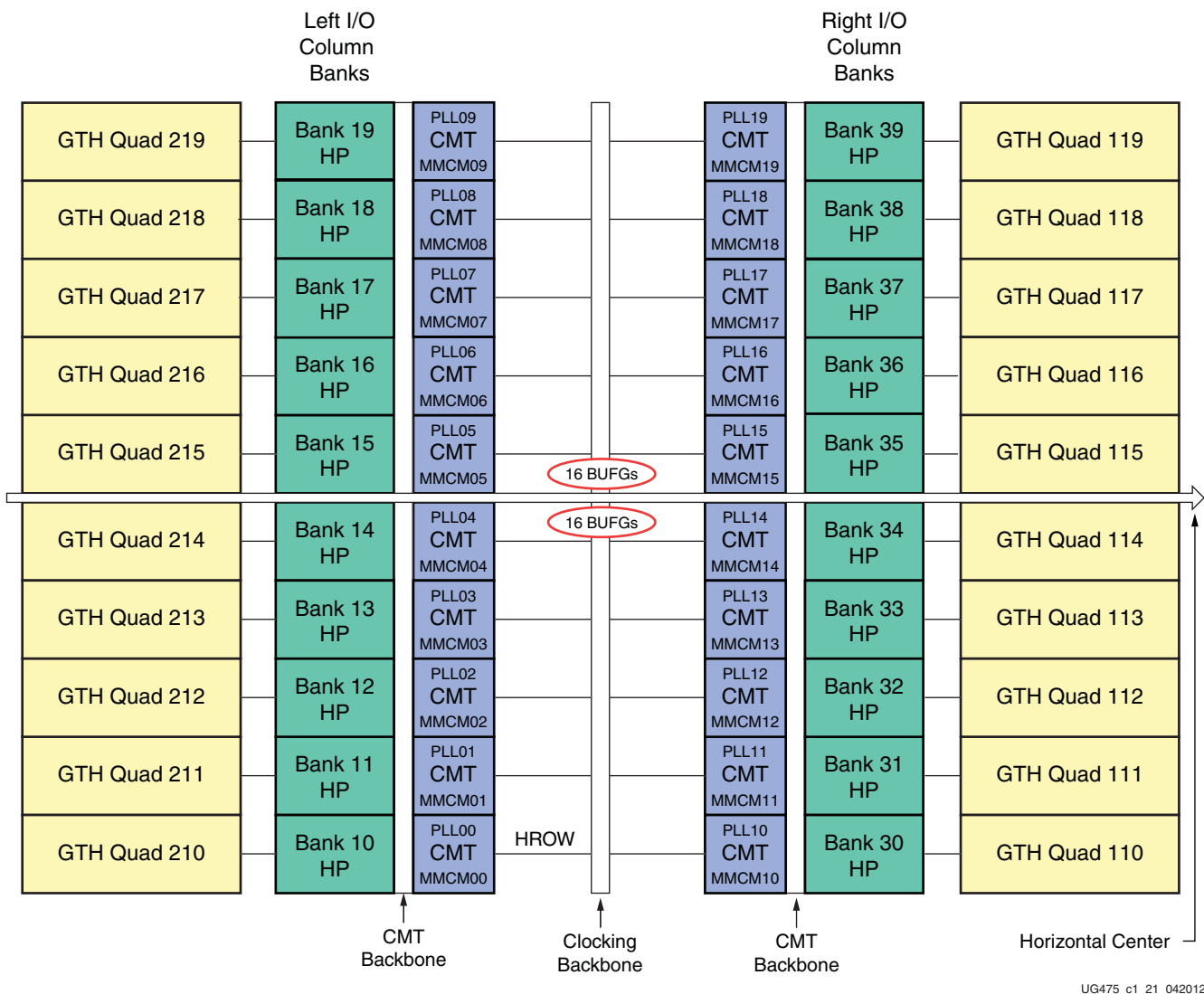
Figure 1-23: XC7VX550T Banks
