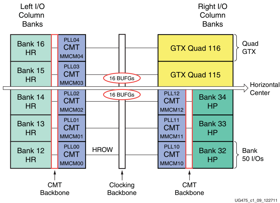
Figure 1-12: XC7K160T Banks
