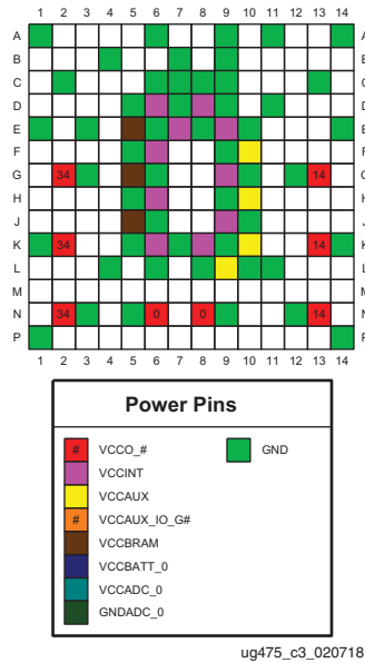
Figure 3-8: FTGB196 Package—XC7S6, XC7S15, XA7S6, and XA7S15 Power and GND Placement
