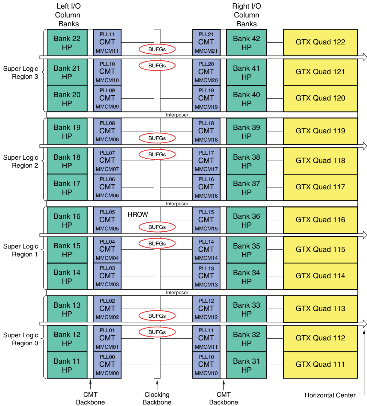
Figure 1-19: XC7V2000T Banks
