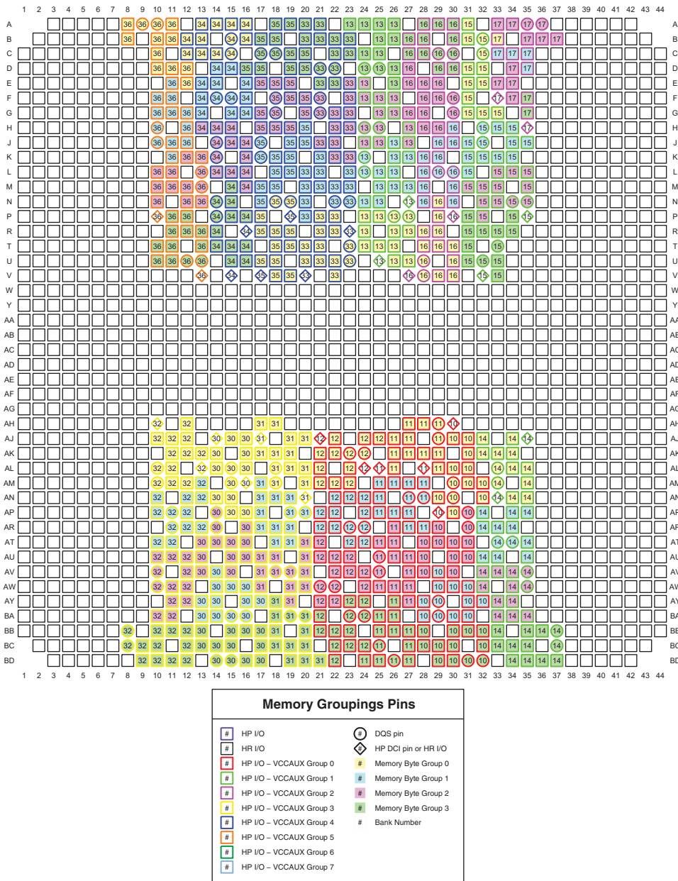
Figure 3-211: FL1926 and FLG1926 Packages—XC7VX1140T Memory Groupings
