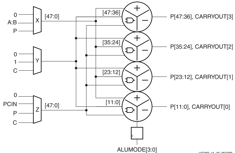
Figure 1-16: Four 12-Bit SIMD Adder Configuration
