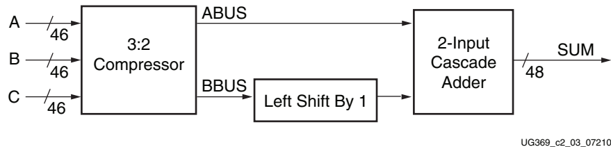
Figure 2-3: Three-Input Adder
