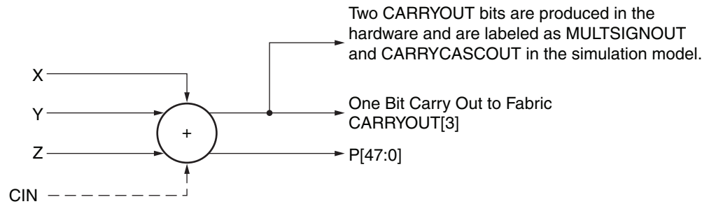
Figure A-4: DSP48E1 Three-Input Adder
