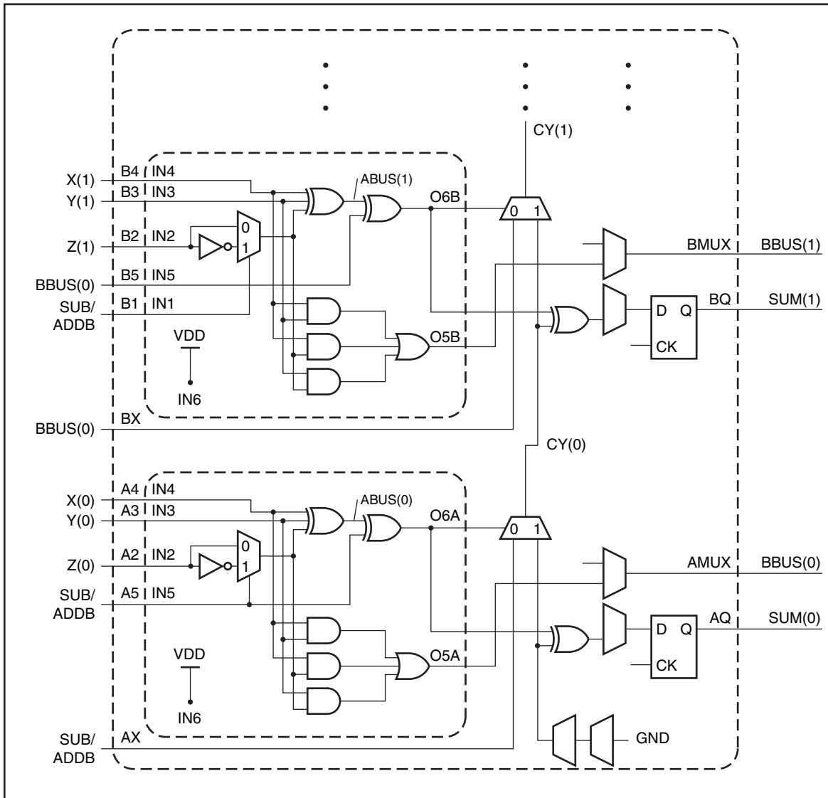
Figure 2-2: Ternary Add/Sub with 3:2 Compressor
