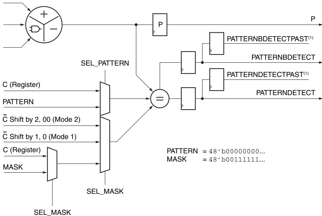
Figure 1-17: Pattern Detector Logic
