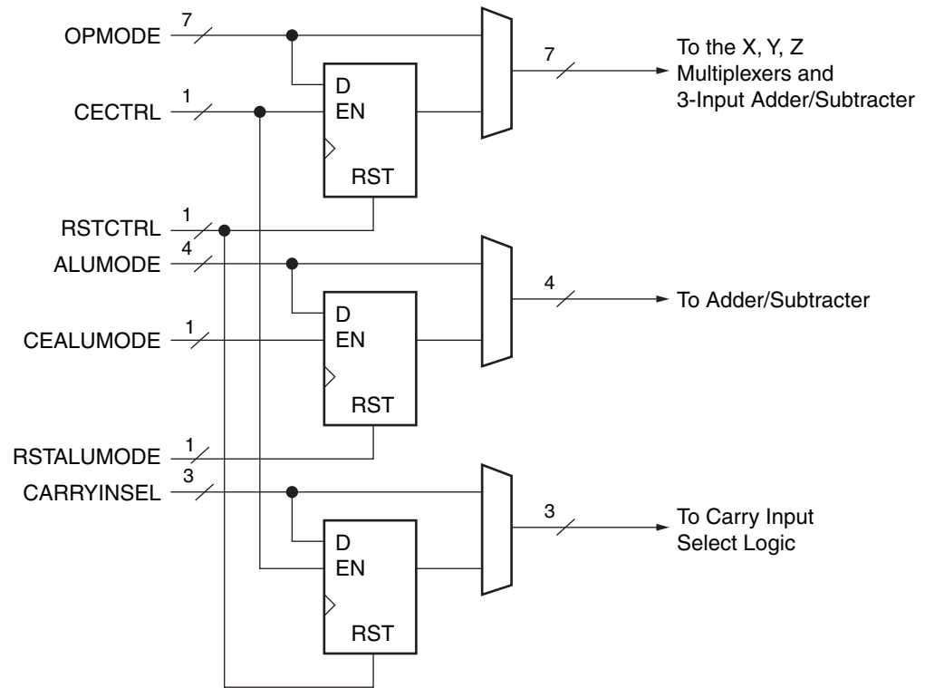
Figure 1-10: OPMODE, ALUMODE, and CARRYINSEL Port Logic
