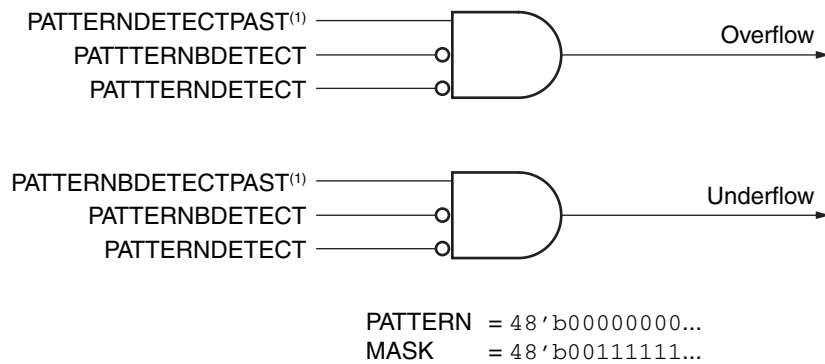
Figure 1-18: Overflow/Underflow Logic in Pattern Detect
