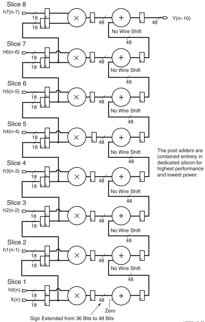
Figure 2-5: Adder Cascade
