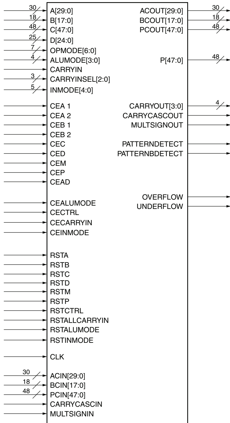
Figure 1-4: DSP48E1 Slice Primitive
