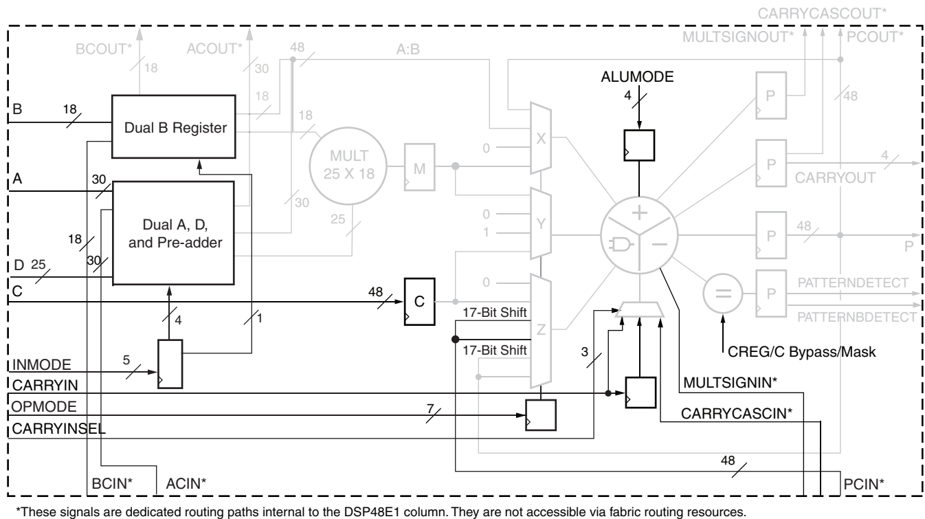
Figure 1-6: Input Ports in the DSP48E1 Slice
