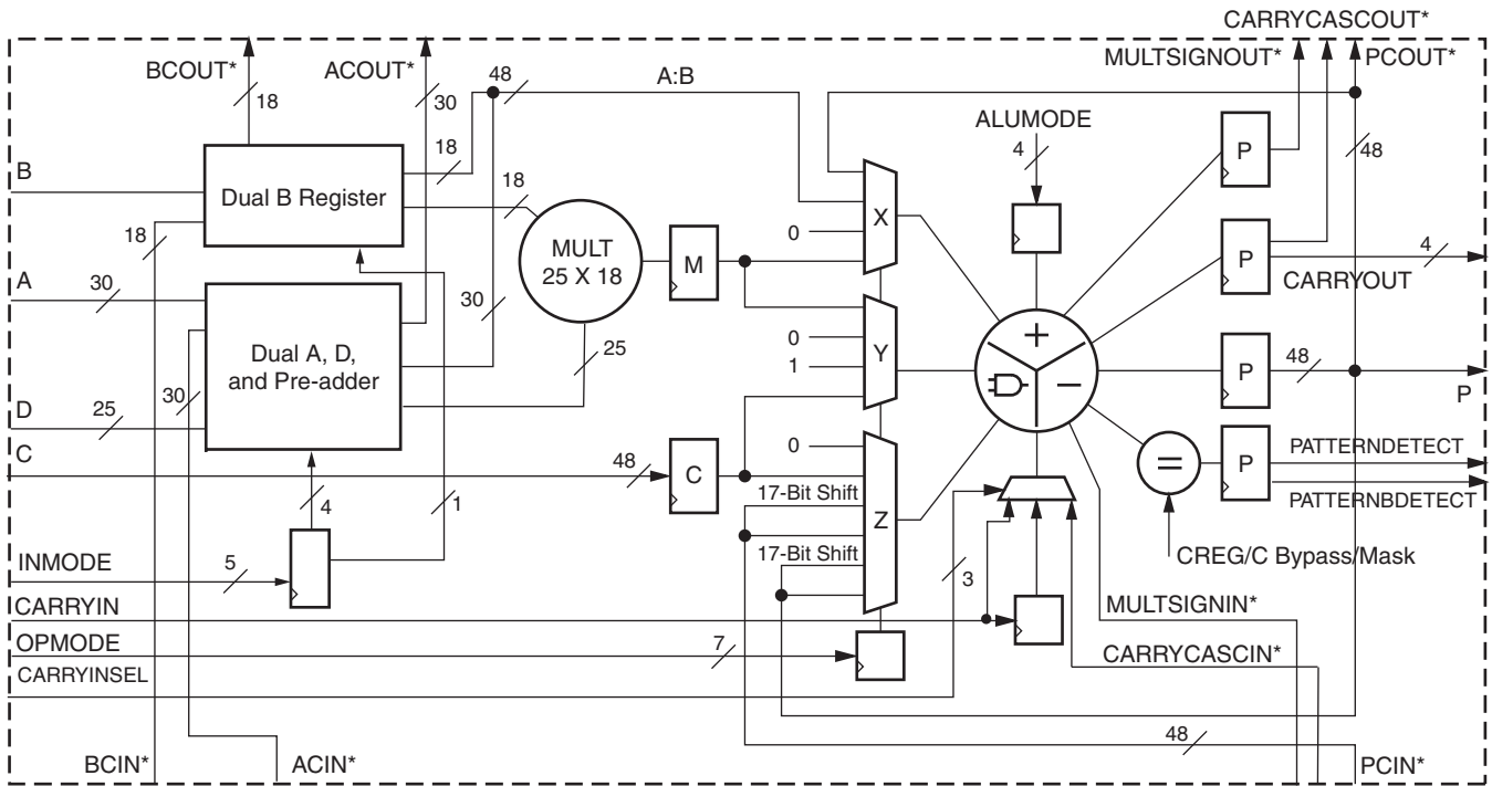
Figure 1-1: Virtex-6 FPGA DSP48E1 Slice
