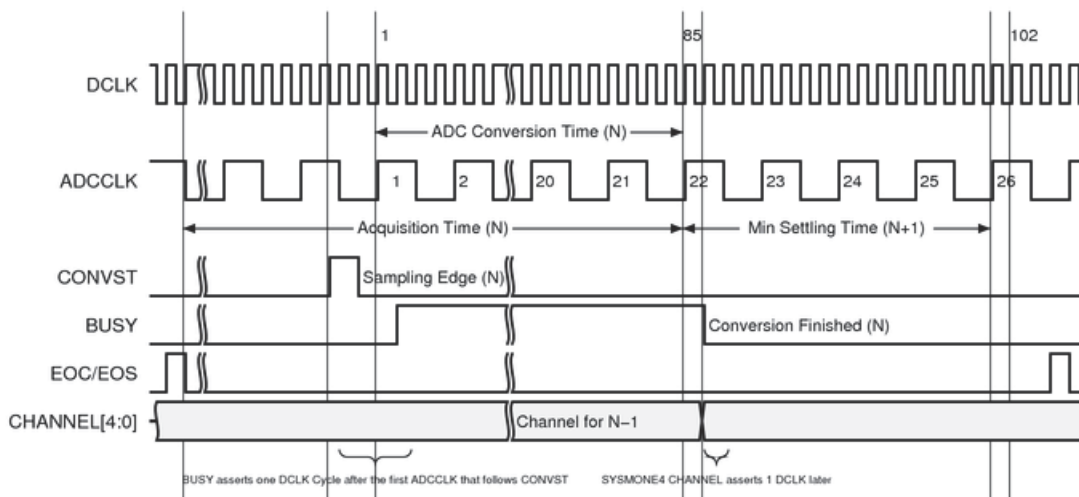
Figure 2-6: Event-Driven Sampling Mode
