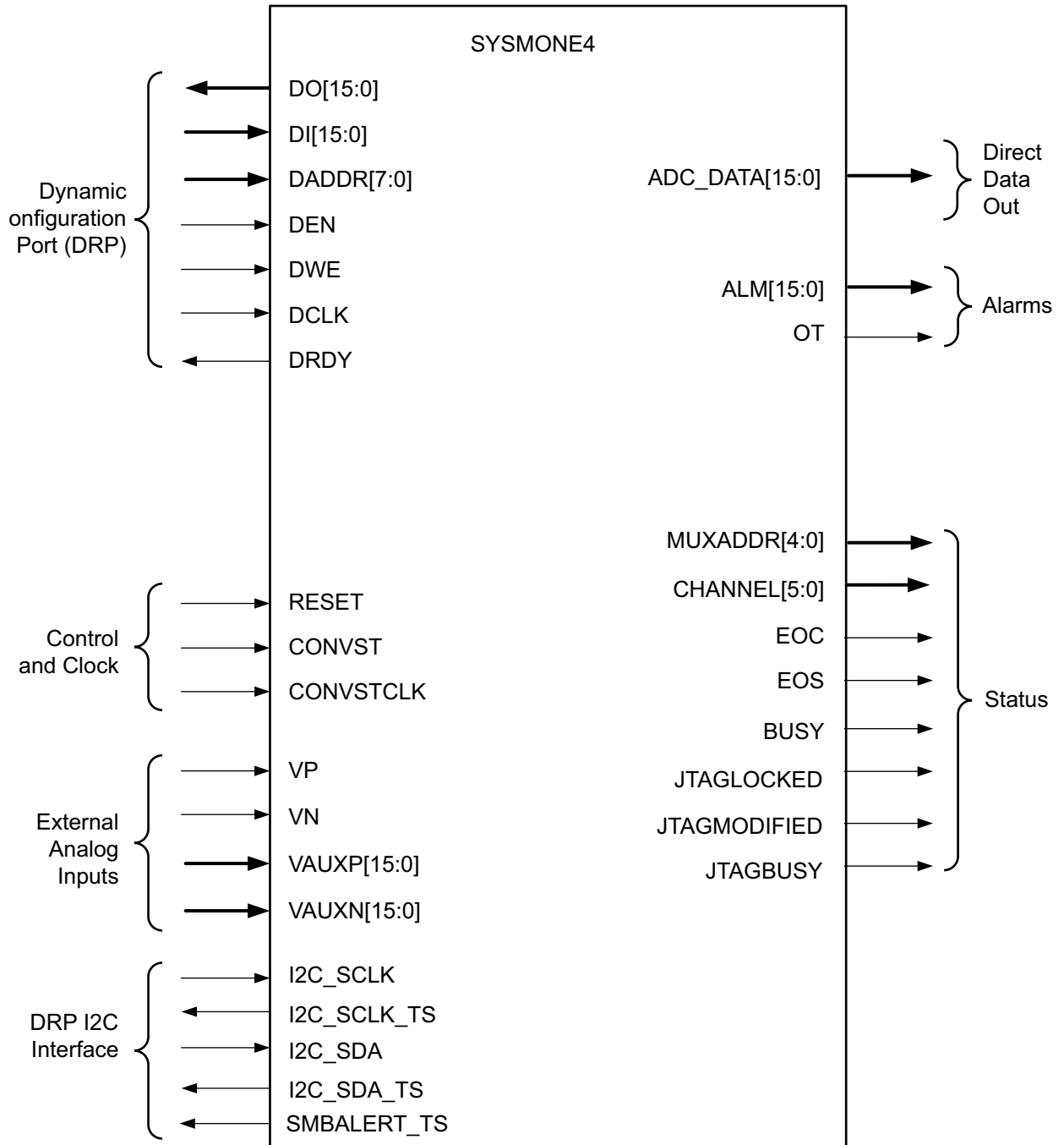
Figure 1-5: SYSMONE4 Primitive Ports
