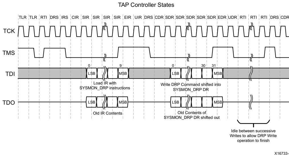
Figure 3-8: SYSMON JTAG DRP Write
