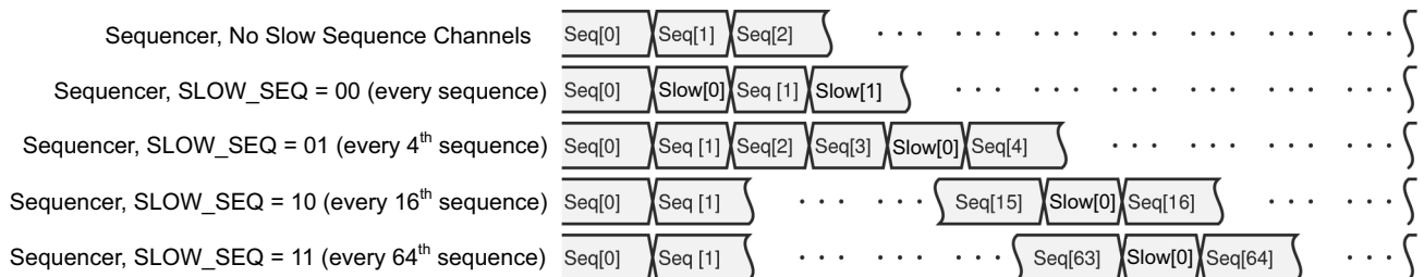
Figure 4-1: Slow Sequence Comparison
