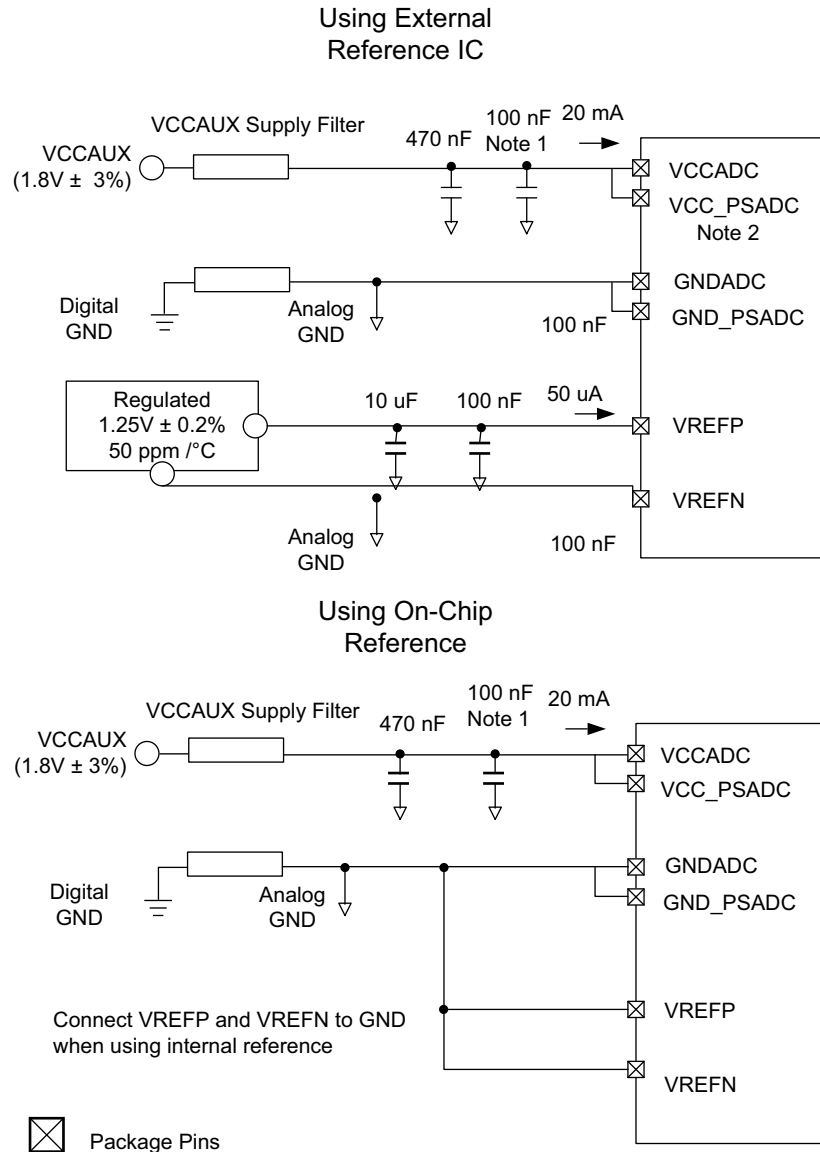
Figure 5-1: ADC Power and Ground Connections
