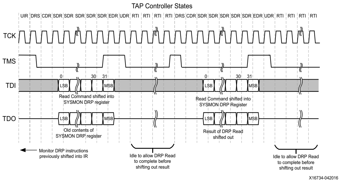
Figure 3-9: SYSMON JTAG DRP Read
