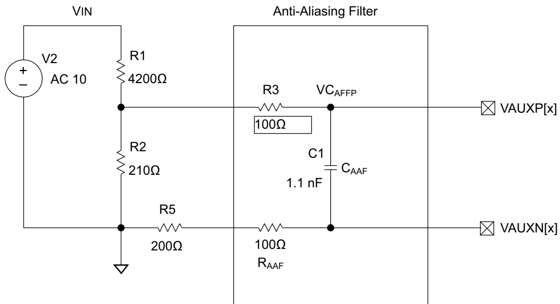
Figure 5-3: Voltage Attenuation
